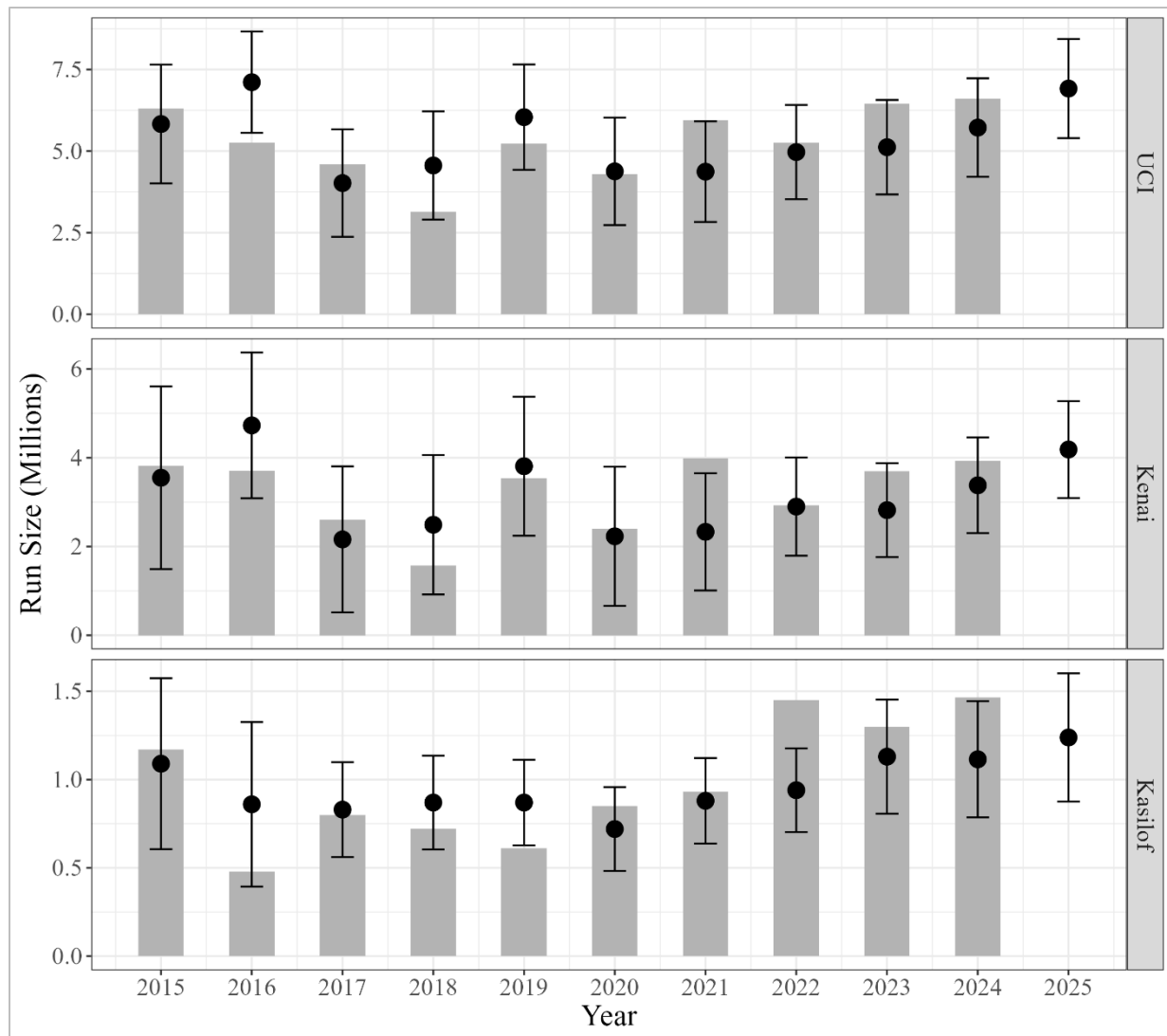
Figure 1. – Estimated total runs (grey bars) of Upper Cook Inlet (top panel), Kenai River (middle panel), and Kaslof River (bottom panel) sockeye salmon compared to total run forecasts (black points), 2015–2024 and 2025 forecast. Error bars represent 80% confidence intervals of forecasts.
